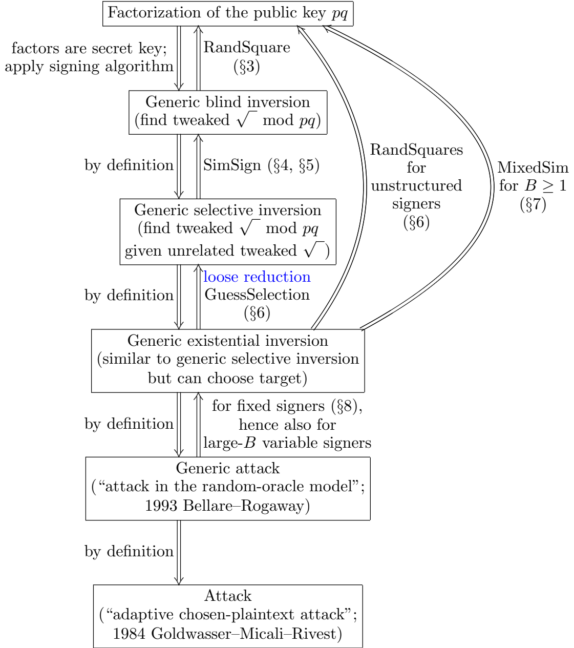
Fig. 0.2. Proven reductions among various types of attacks against Rabin–Williams signatures. SimSign is more difficult for Rabin–Williams than for RSA; the unstructured case was outlined in 1996 Bellare–Rogaway, but the principal case was specifically prohibited in 1996 Bellare–Rogaway and requires extra work performed in this paper. GuessSelection is standard but not tight. MixedSim is tight; it combines the new simulator with the central idea of 2003 Katz–Wang. RandSquares is also new in this paper, and also tight; it can be viewed as the result of eliminating guesses from RandSquare(SimSign(GuessSelection)), or as the result of eliminating aborts from an overgeneralization of MixedSim.
