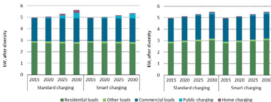
Figure 20 • Impact of electric car deployment on a generic local grid in the European Union, B2DS (left) and 2DS (right)
