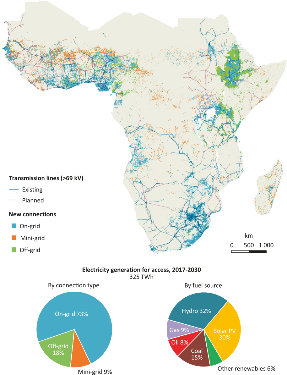
Figure 4.9 ▶ New connections and power generation for electricity access in sub-Saharan Africa in the New Policies Scenario, 2017-2030
