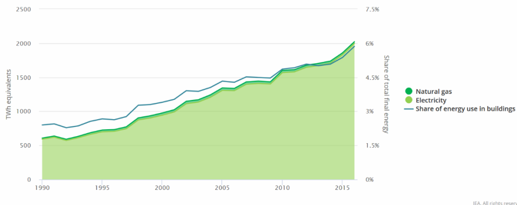
Figure 40: Energy use from cooling worldwide [81]
