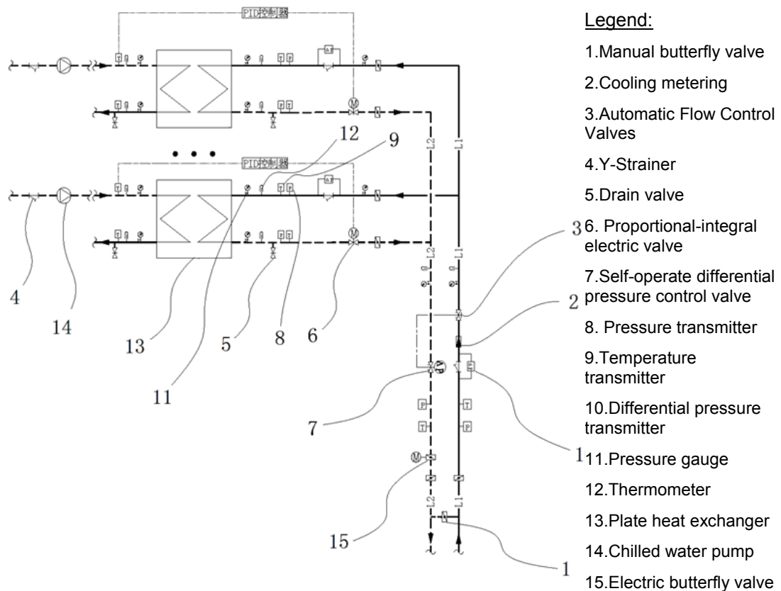
Figure 25: Installation of meters and valves of heat exchangers in ETS
