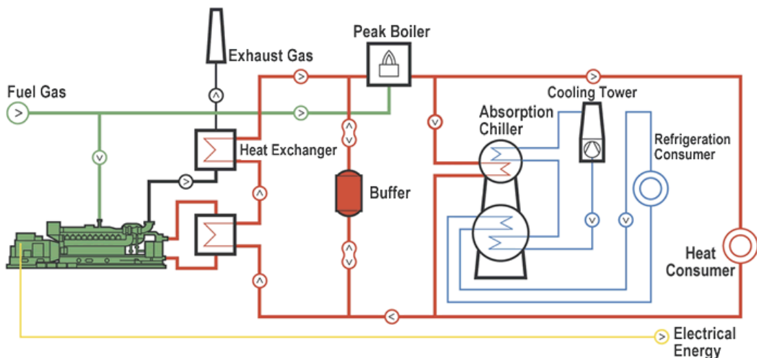
Figure 7: Trigeneration scheme [21]
