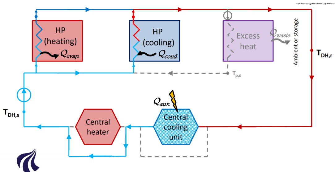
Figure 34: Principle scheme (summer)
