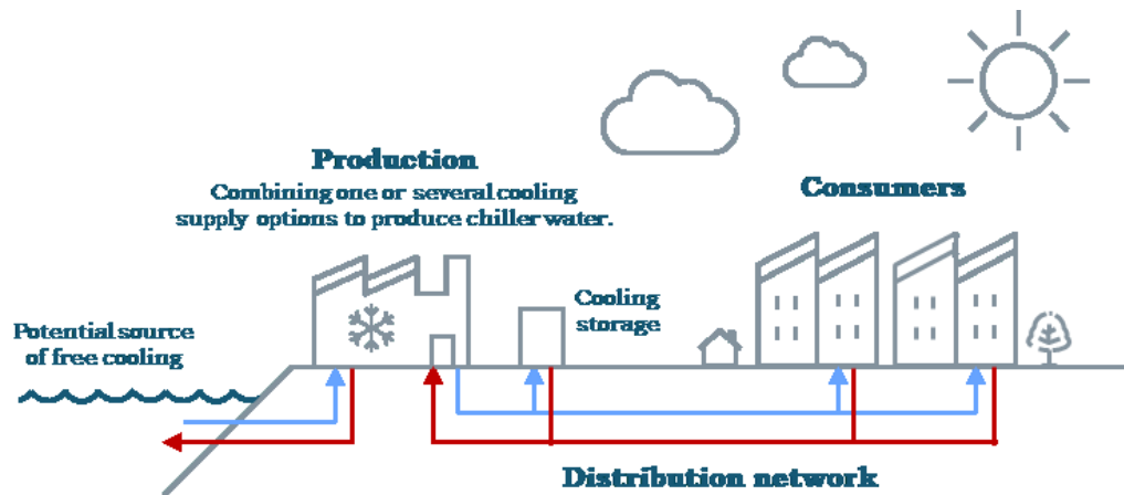
Figure 5: The general principle of DC operation.
