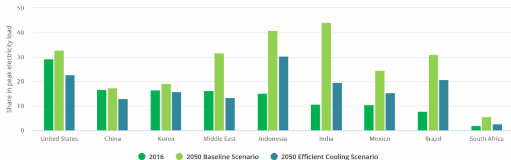
Figure 42: Share of cooling in electricity peak loads [83]
