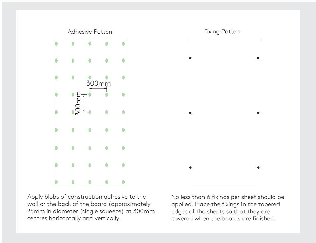
Figure 11 – Construction Adhesive Pattern
