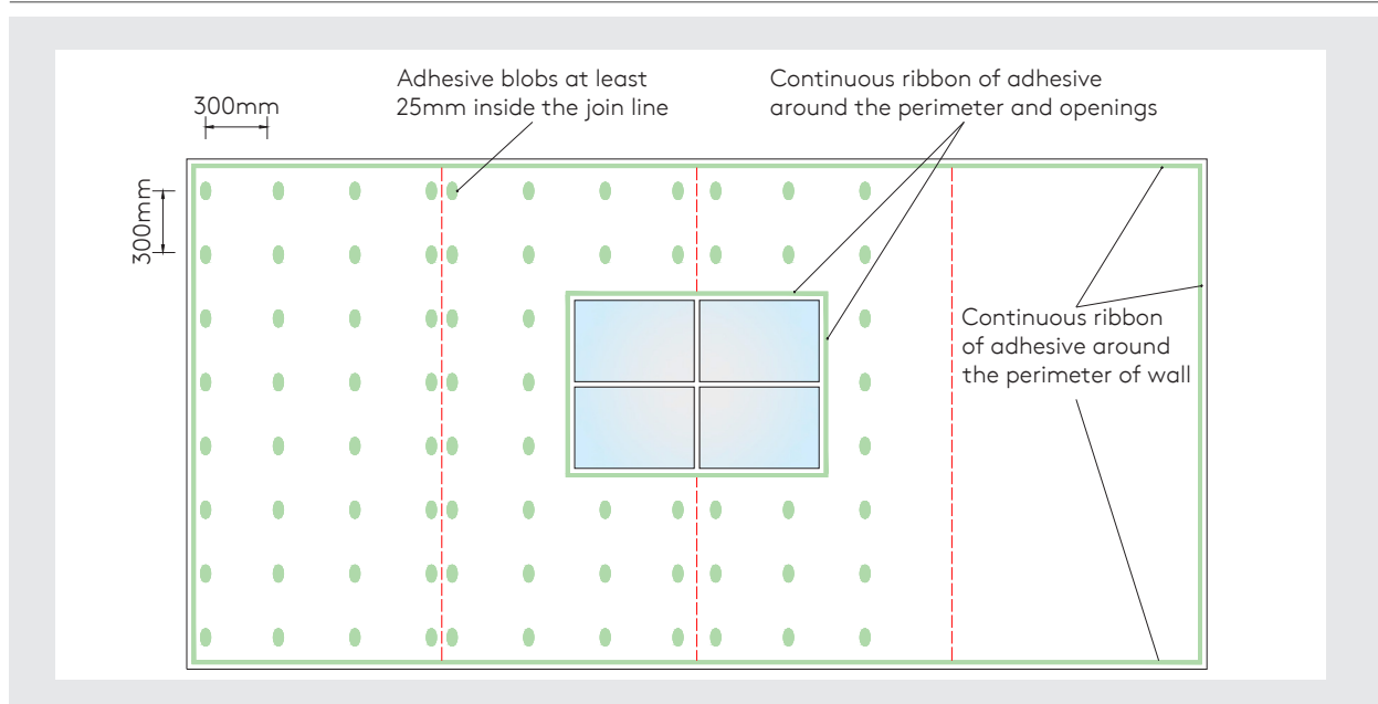
Figure 6 – Adhesive Blobs & Chalk Line Pattern
