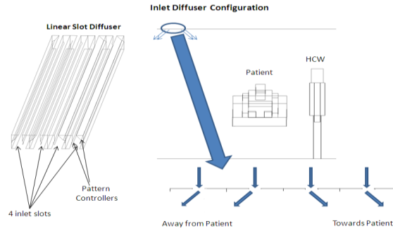
Figure 2. Inlet diffuser design
