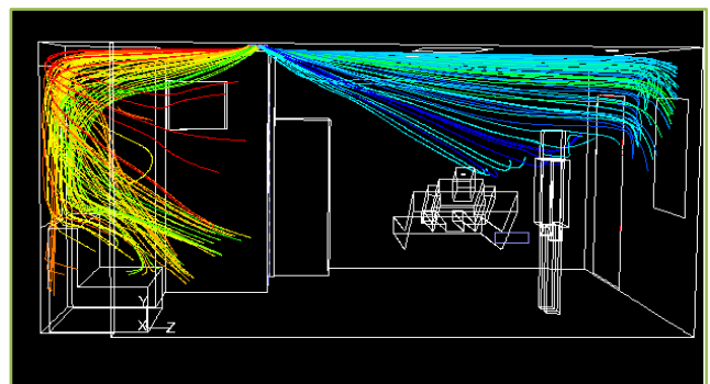
Fig. 4. Pathlines, colored by origination location in AIIR Fig. 5. Pathlines, colored by origination location in patient room
