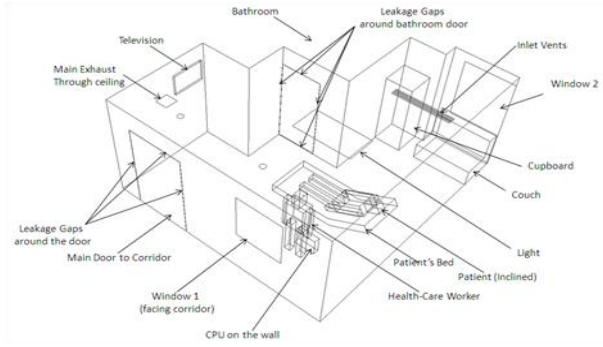
Figure 1. Isometric view of the AIIR
