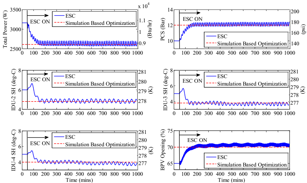
Figure. 5. Input and output trajectories for multi-variable ESC control of 1H3C mode.
