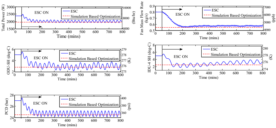
Figure 7. Input and output trajectories for multi-variable ESC control of 3H1C mode.
