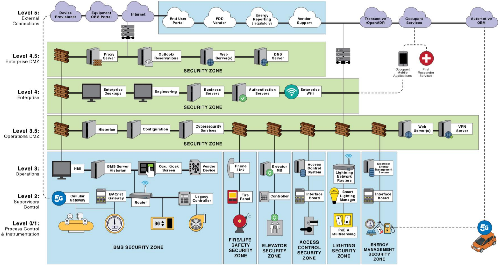
Figure 1. Commercial Building Reference Architecture
