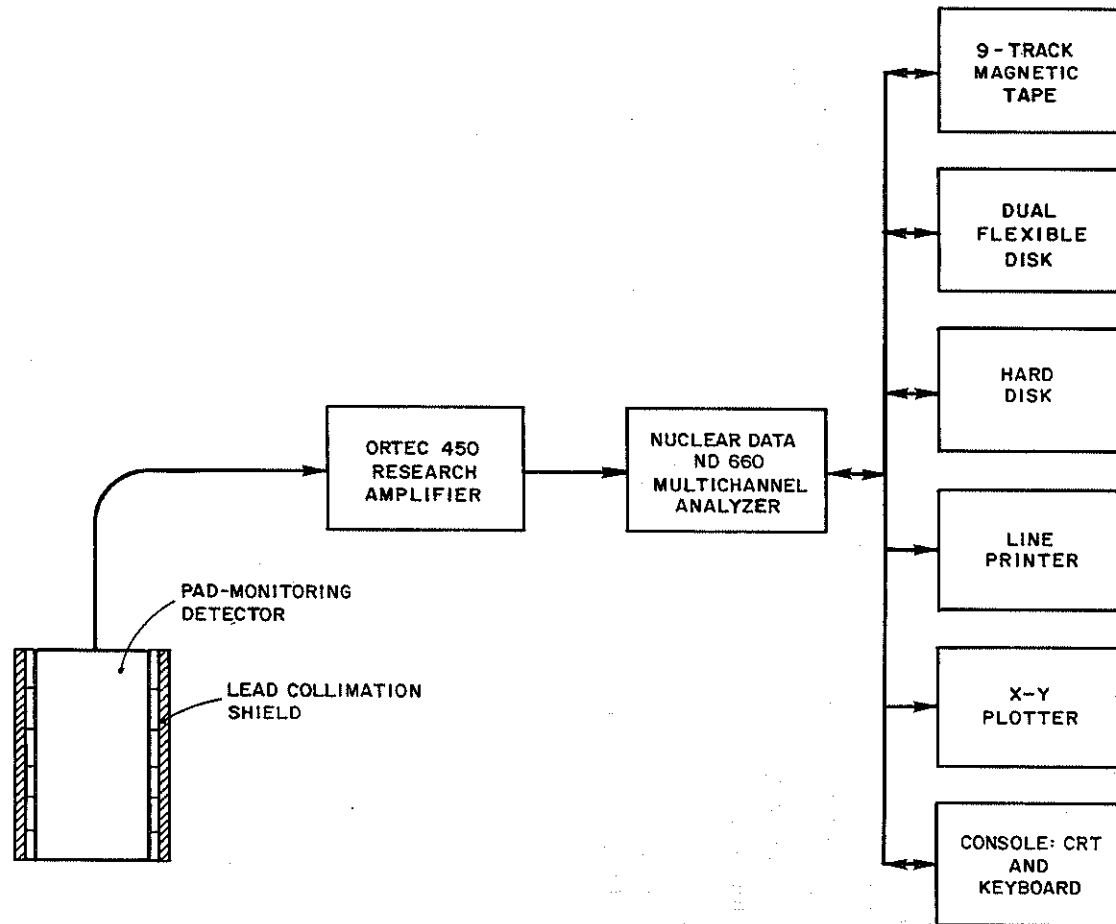
Figure 7-1. Block Diagram of CFMS Pad-Monitoring Detector System
