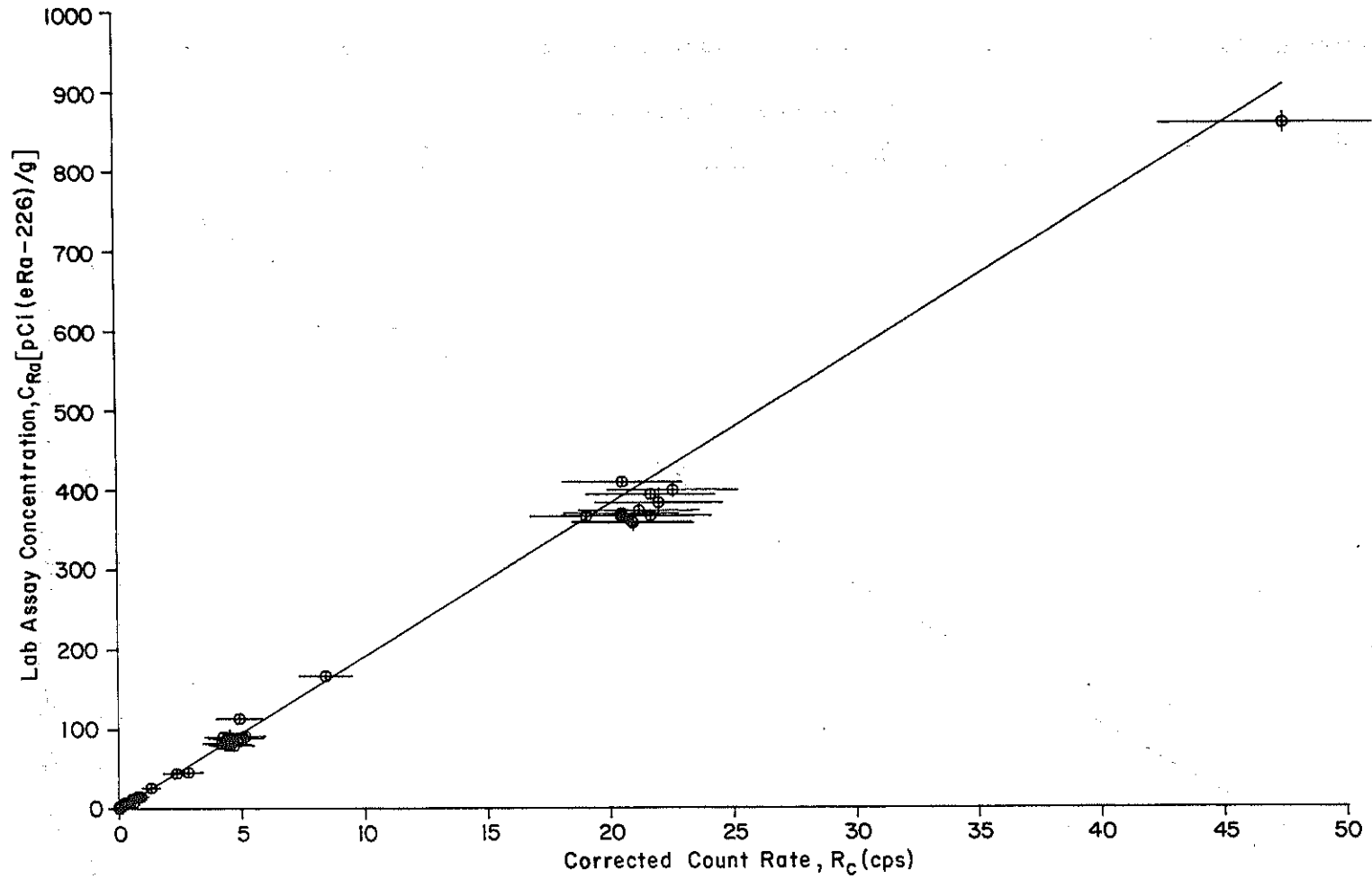
Figure 6-2. Regression of Corrected Count Rate Versus Laboratory Assay Concentration for Radium
