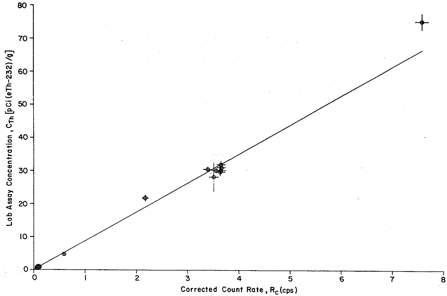
Figure 6-3. Regression of Corrected Count Rate Versus Laboratory Assay Concentration for Thorium
