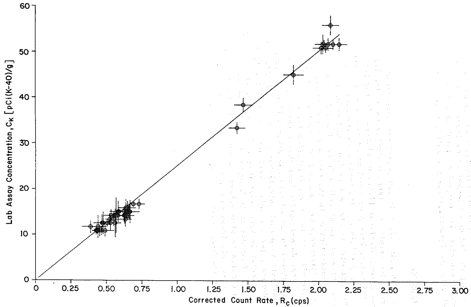
Figure 6-1. Regression of Corrected Count Rate Versus Laboratory Assay Concentration for Potassium
