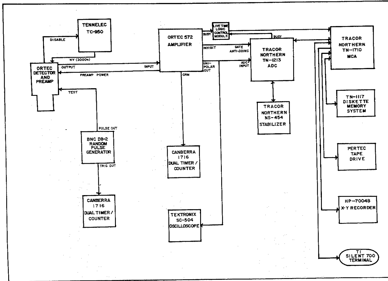
Figure 3-1. Block Diagram of Mobile Gamma-Ray Spectroscopy System with ORTEC HPGe Portable Germanium Detector
