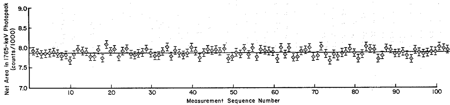
Figure 3-4. Sensitivity of the Germanium Detector to a 1- \mu Ci Ra-226 Source
