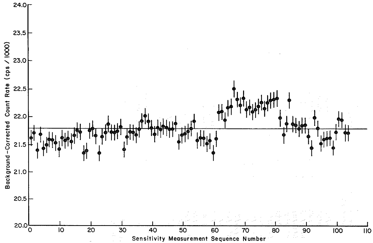
Figure 7-4. Sensitivity of the CFMS Sodium Iodide Detector to a Ra-226 Source
