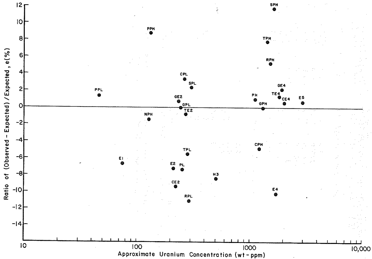
Figure 7-6. Plot of the Percentage Difference Between Observed and Expected Count Rates Versus Uranium Concentration for the Radium-Enriched Pads
