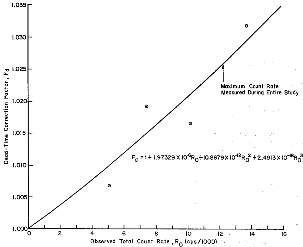
Figure 7-5. Dead-Time Correction Factor Versus Total Count Rate for the CFMS
