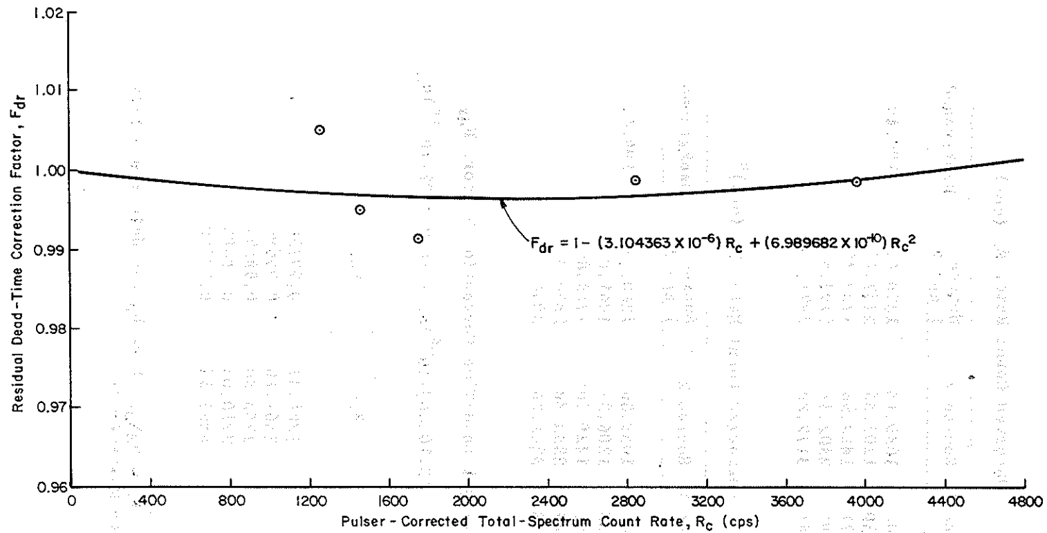
Figure 3-2. Pulser Dead-Time Verification
