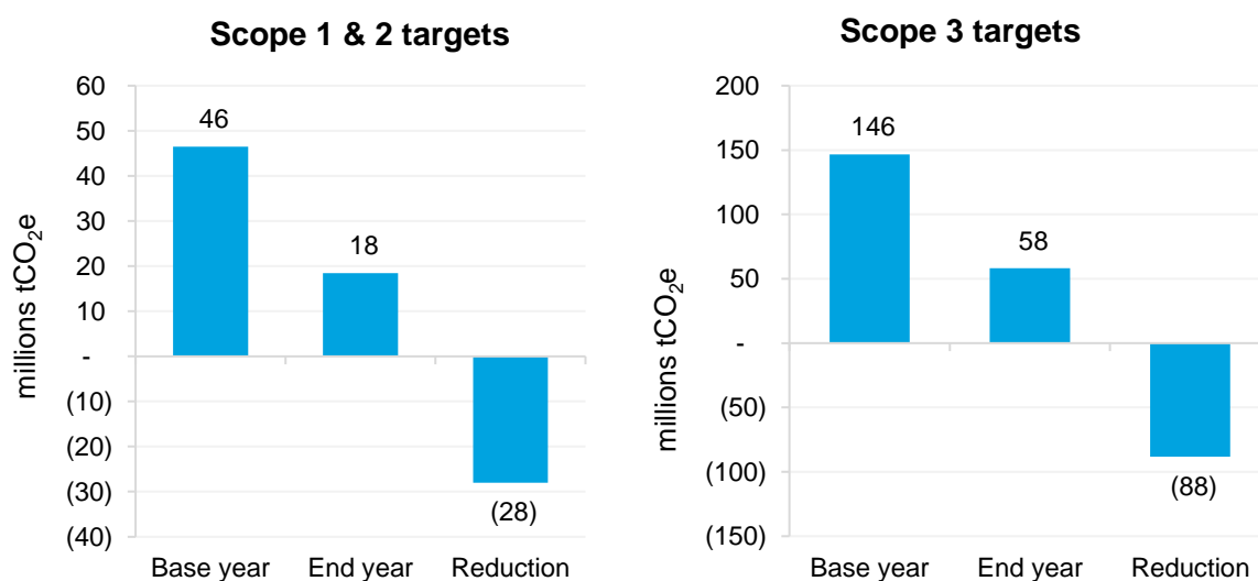
Figure 3.7: Measurable emissions target reductions by 2030, millions tCO 2 e
